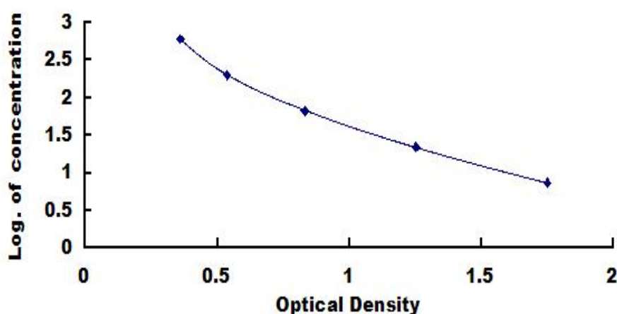
Typical Standard Curve for VB2 ELISA.
