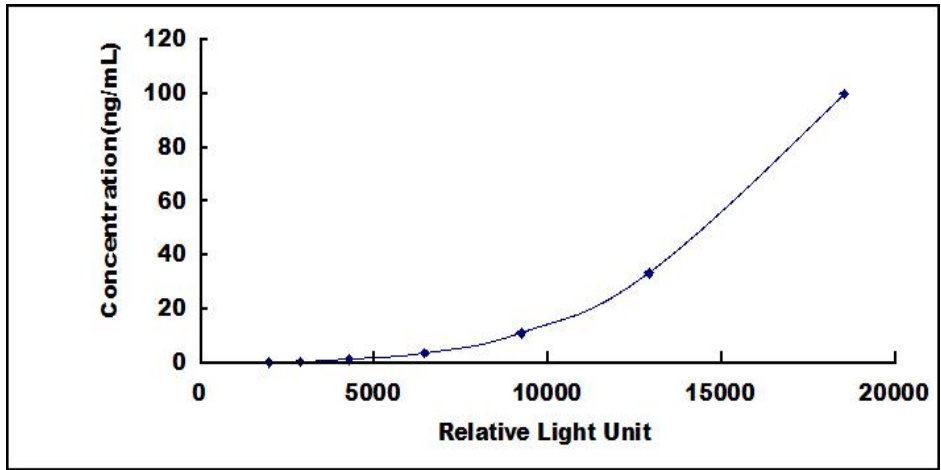
Typical Standard Curve for Hsp60 ELISA.
