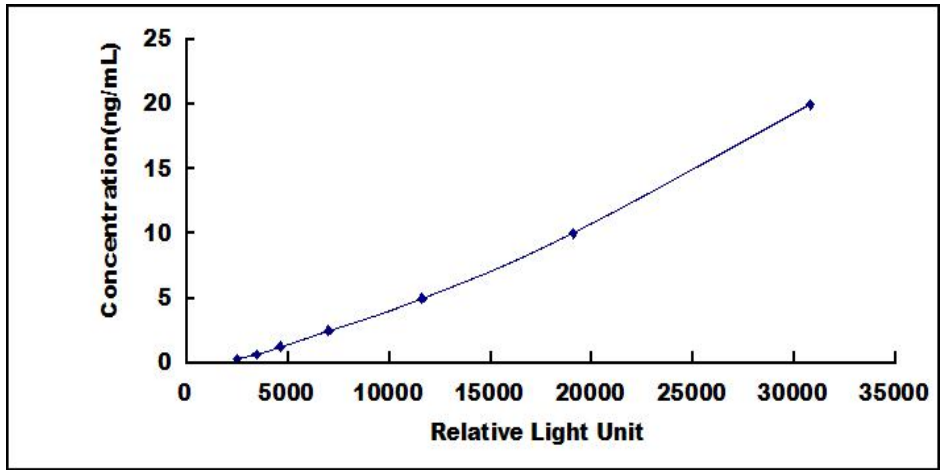
Typical Standard Curve for DEFa1 ELISA.
