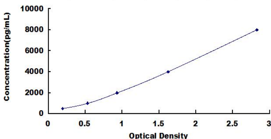
Typical Standard Curve for MHCDMb ELISA.
