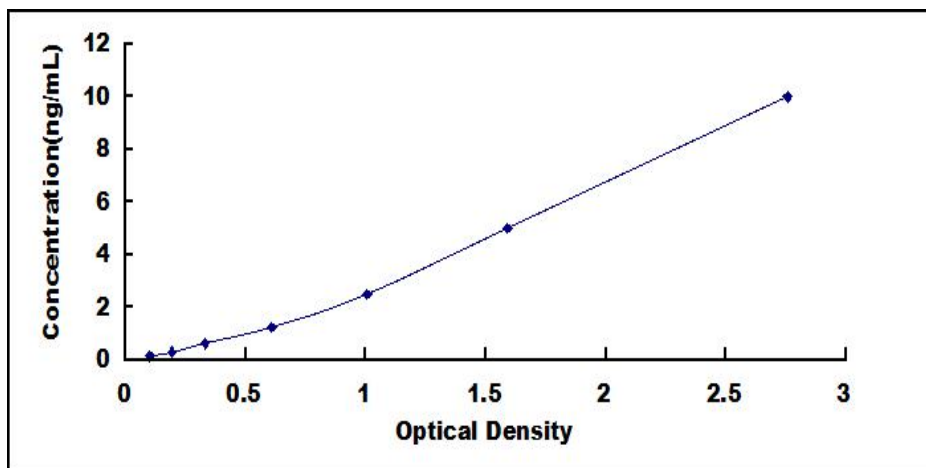
Typical Standard Curve for KAT2B ELISA.
