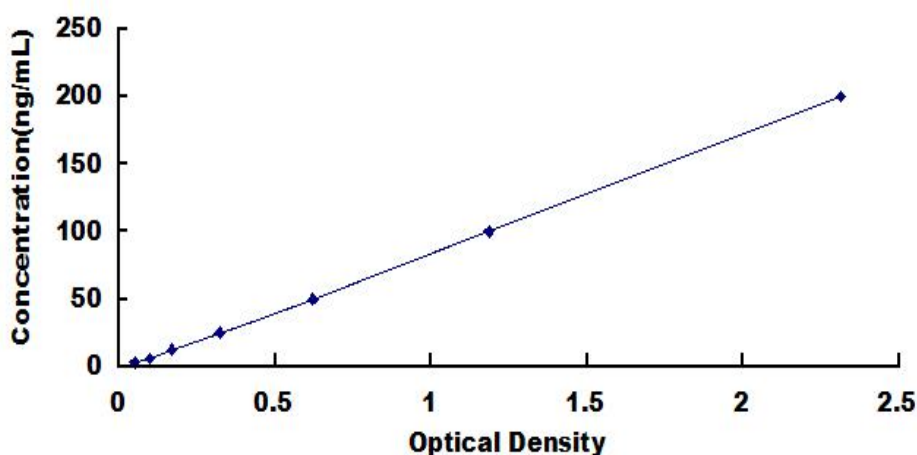
Typical Standard Curve for SELENBP1 ELISA.
