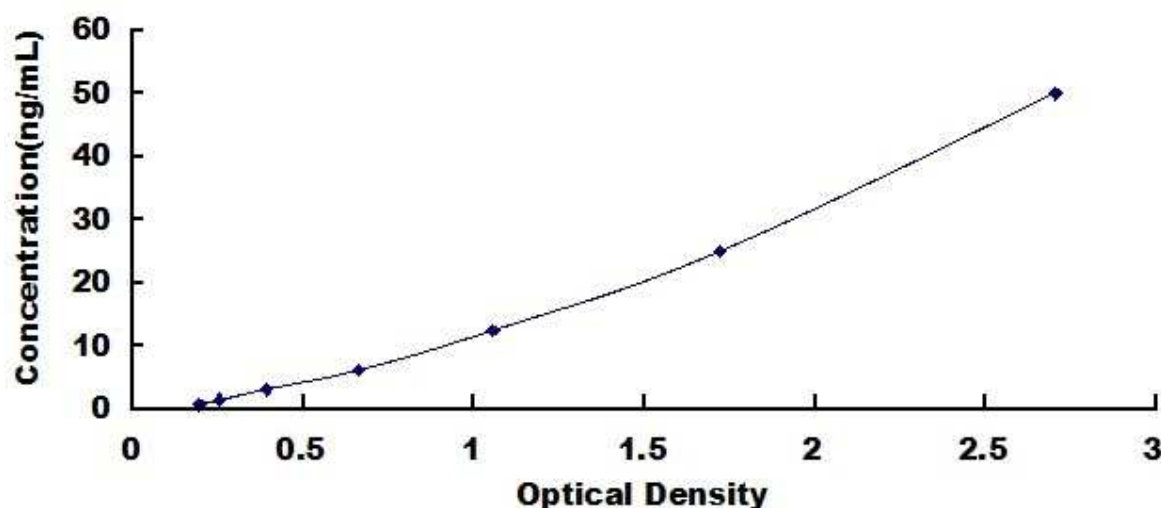
Typical Standard Curve for CKMT2, Rat ELISA.
