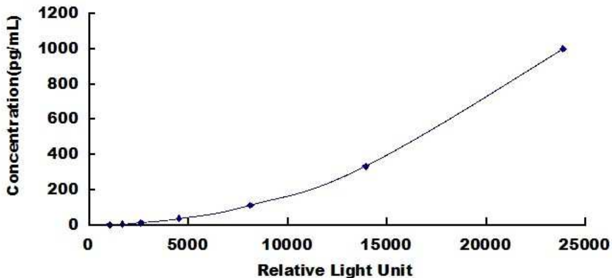
Typical Standard Curve for NEFL, Human CLIA.
