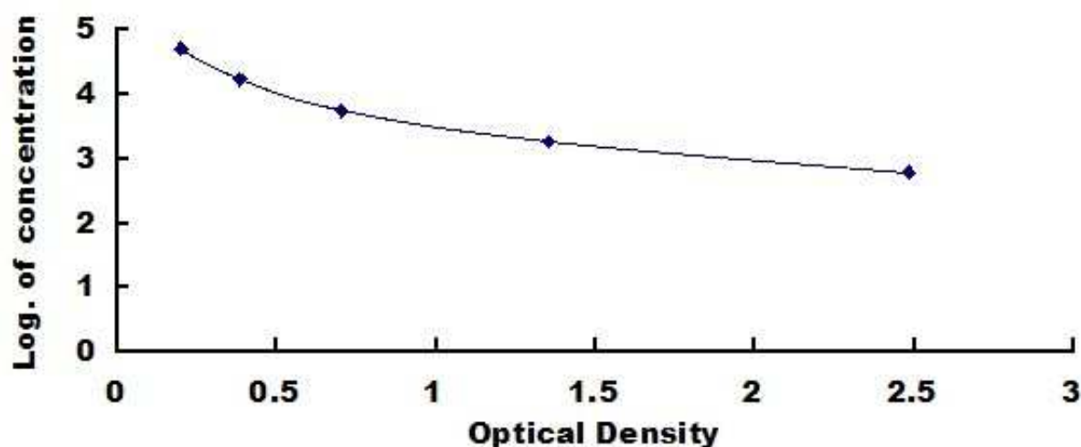
Typical Standard Curve for Kanamycin ELISA.
