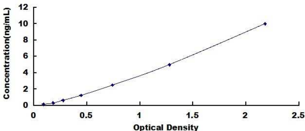
Typical Standard Curve for TNFaIP6, Rat ELISA.
