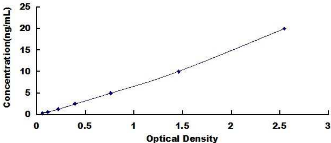
Typical Standard Curve for Myoglobin, Bovine ELISA.
