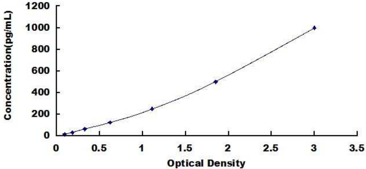
Typical Standard Curve for Tsukushin, Mouse ELISA.
