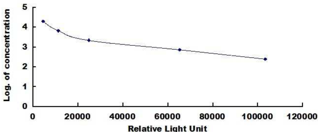
Typical Standard Curve for Free Thyroxine CLIA.
