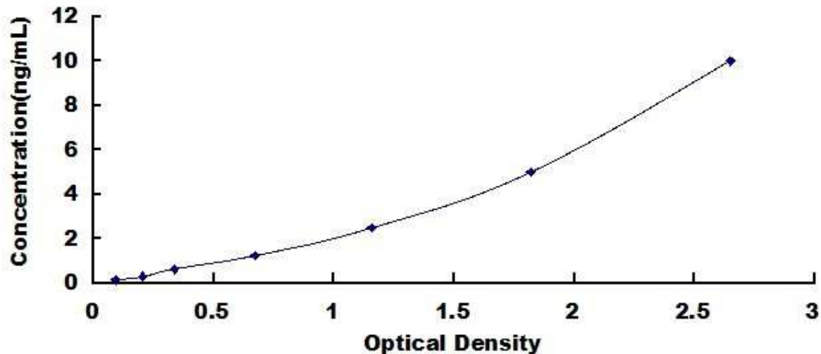
Typical Standard Curve for MYH1, Bovine ELISA.
