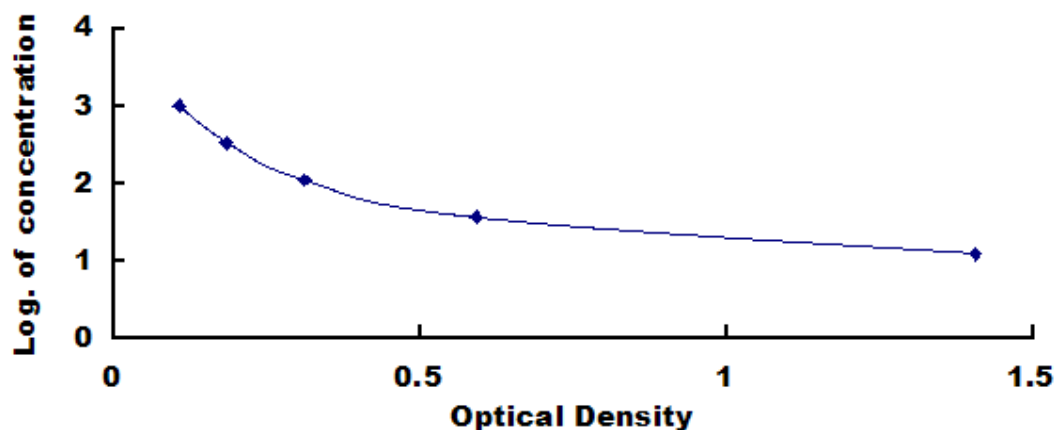
Typical Standard Curve for ACTH, Gallus ELISA.
