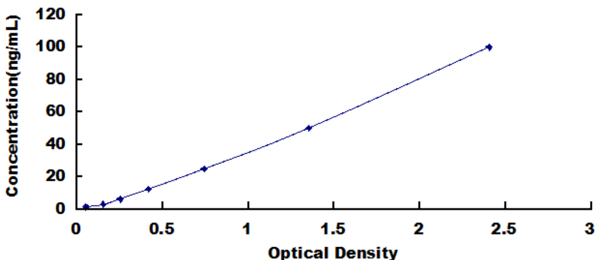
Typical Standard Curve for ALPI, Mouse ELISA.
