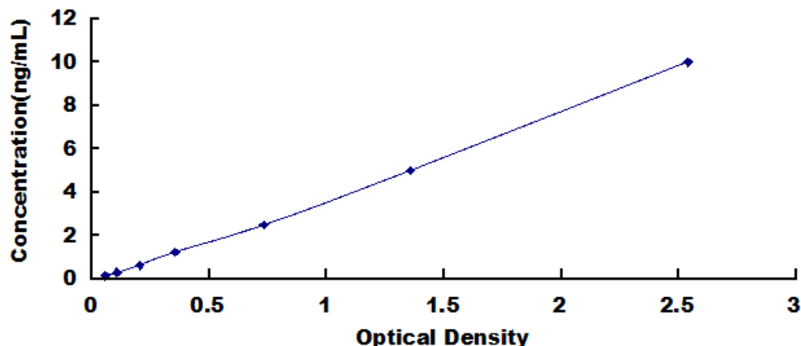
Typical Standard Curve for MAP2K2, Human ELISA.
