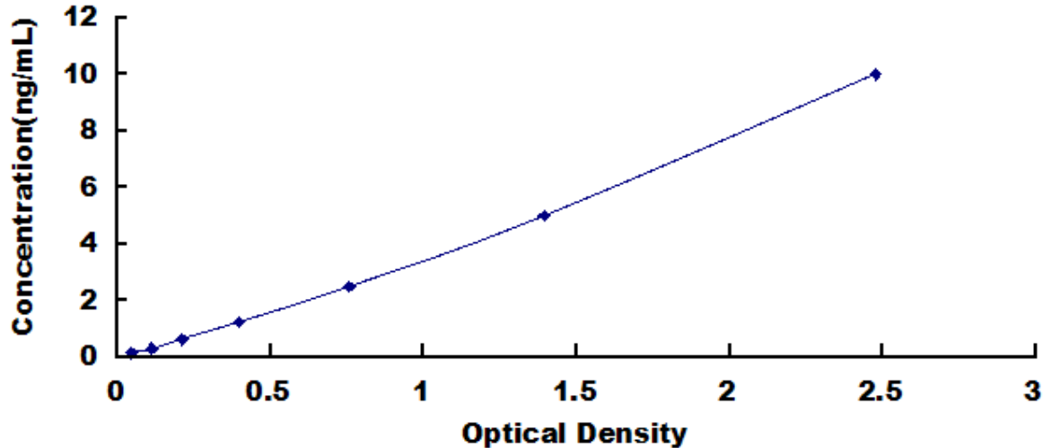
Typical Standard Curve for KBTBD10, Rat ELISA.
