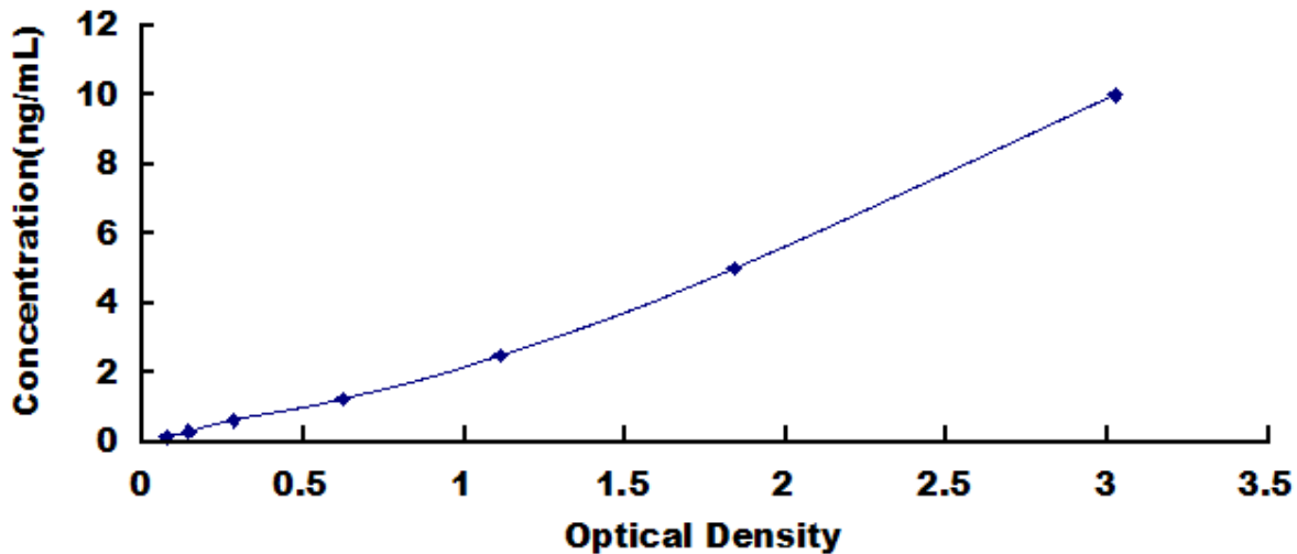
Typical Standard Curve for HSP90b1, Ovine ELISA.
