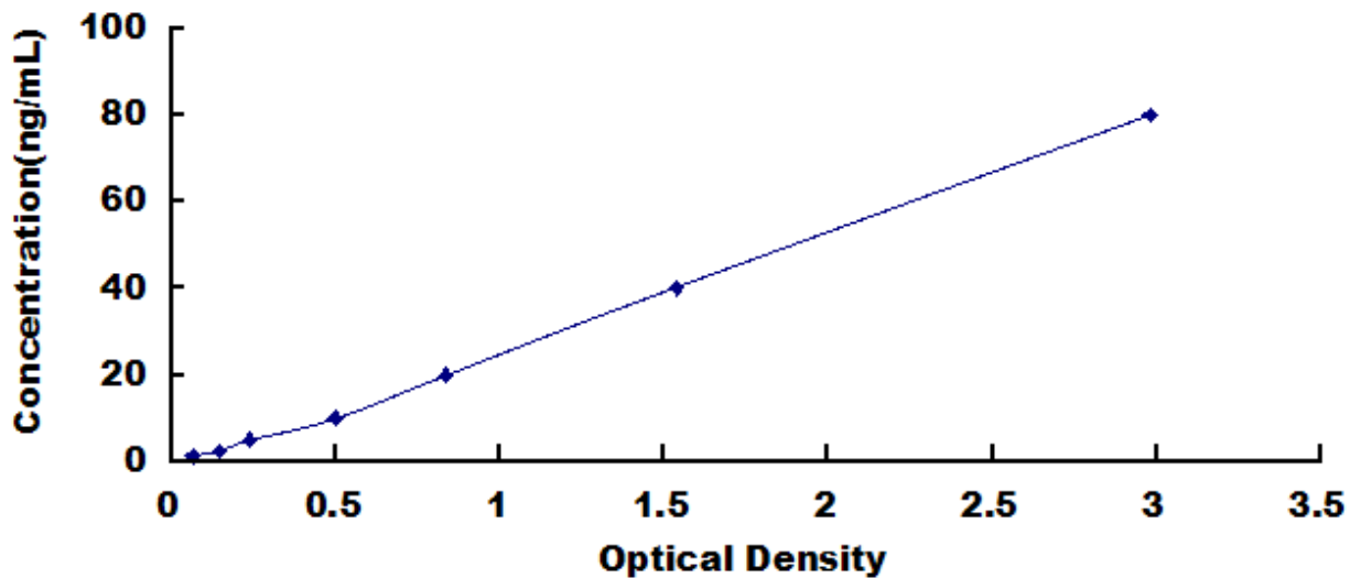
Typical Standard Curve for APOC1, Mouse ELISA.
