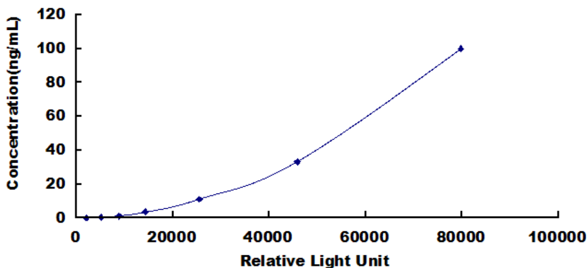
Typical Standard Curve for CALPRO, Canine CLIA.
