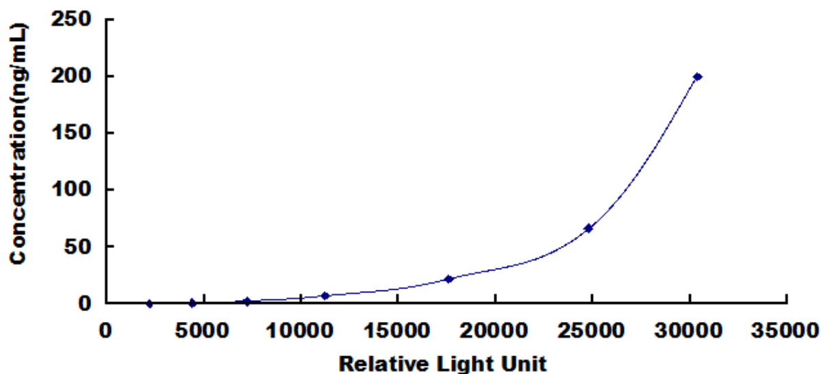
Typical Standard Curve for Elastin, Bovine CLIA.
