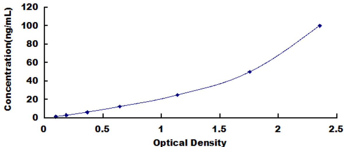
Typical Standard Curve for SDHB, Rat ELISA.
