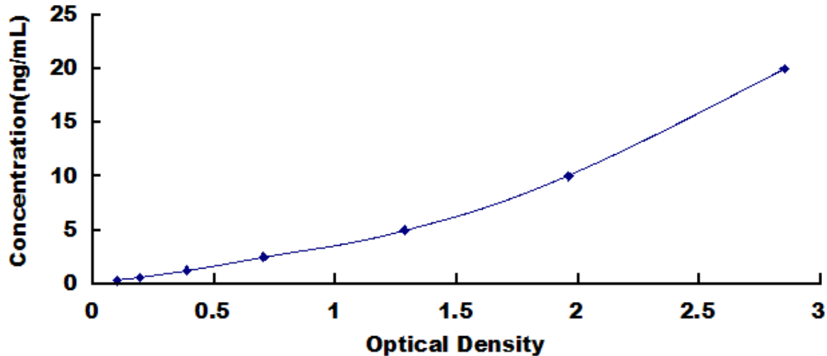
Typical Standard Curve for SOCS3, Bovine ELISA.
