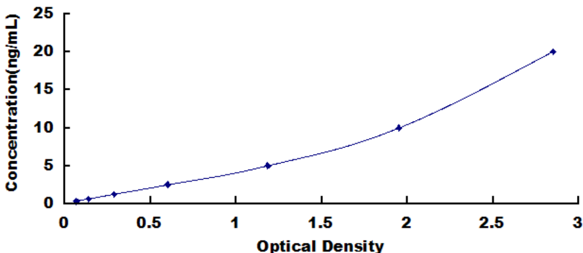
Typical Standard Curve for AMFR, Human ELISA.
