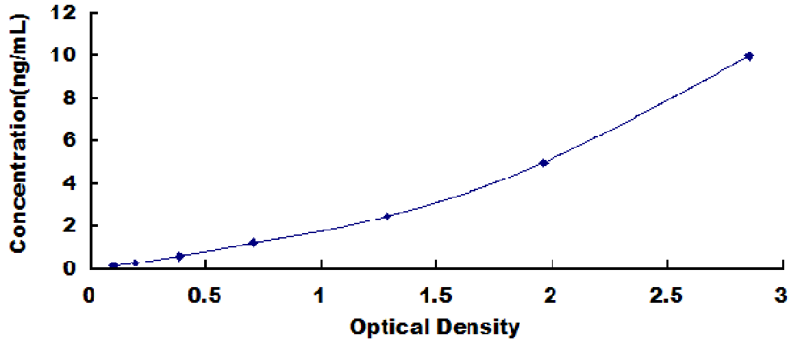
Typical Standard Curve for FGFR4, Mouse ELISA.
