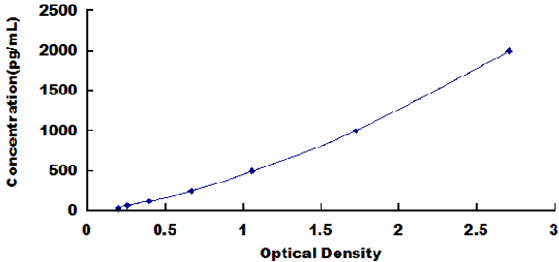
Typical Standard Curve for HIST2H2BE, Human ELISA.
