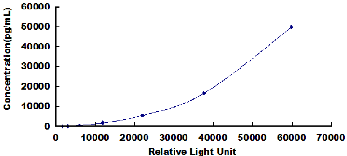
Typical Standard Curve for ROR1, Human CLIA.
