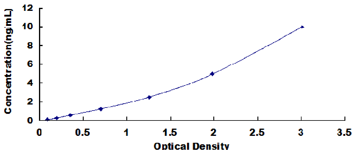
Typical Standard Curve for Bcl2, Porcine ELISA.
