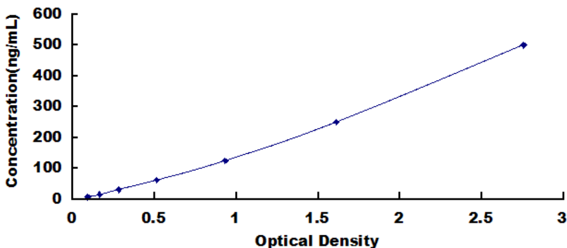
Typical Standard Curve for IgG, Ovine ELISA.
