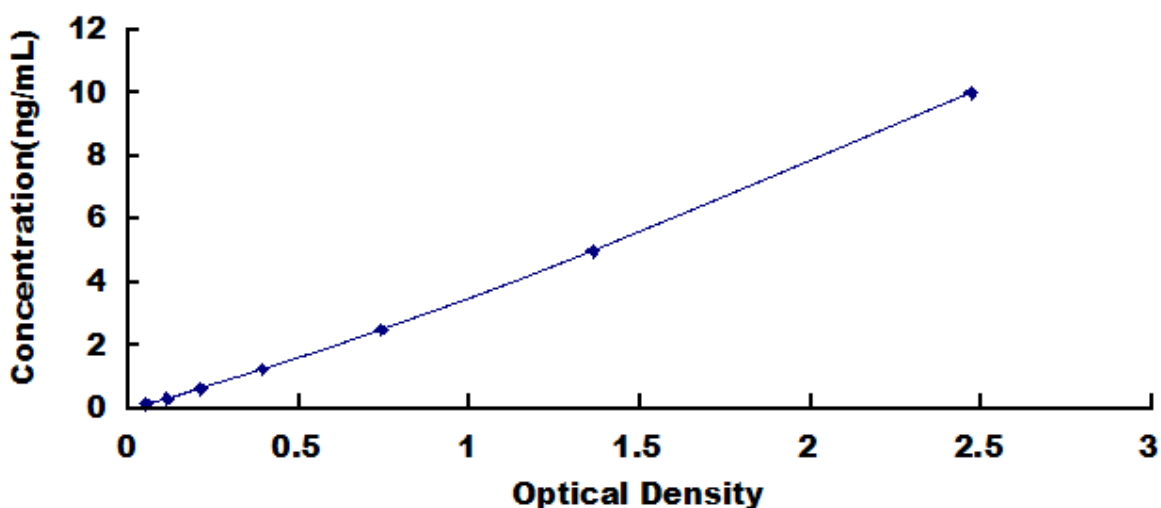
Typical Standard Curve for PL, Mouse ELISA.
