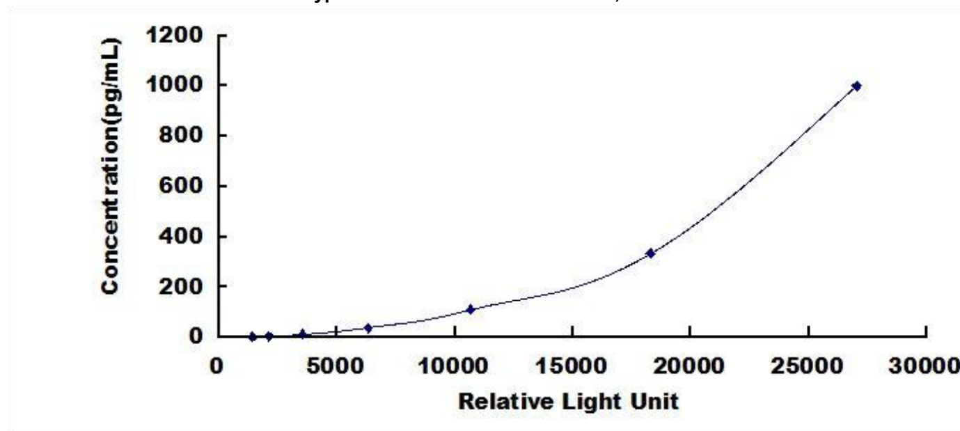
Typical Standard Curve for INHbE, Human CLIA.
