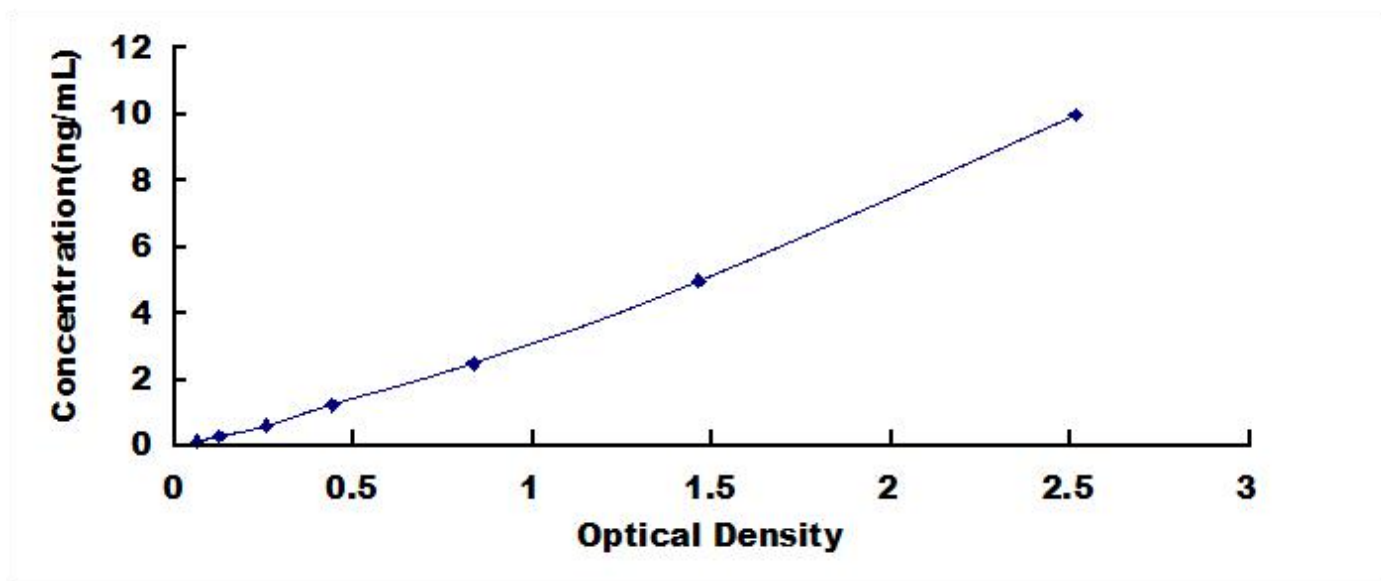
Typical Standard Curve for ANO1, Mouse ELISA.
