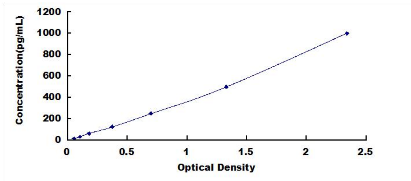
Typical Standard Curve for NGF, Simian ELISA.
