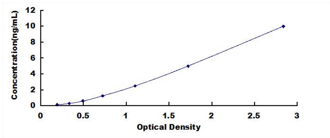
Typical Standard Curve for GFPT1, Human ELISA.
