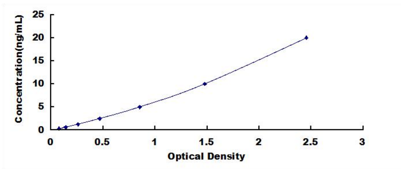
Typical Standard Curve for PGAM2, Mouse ELISA.
