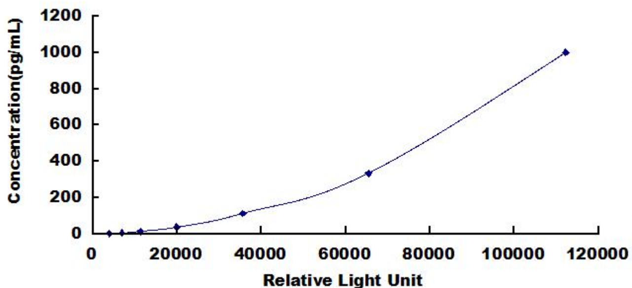
Typical Standard Curve for C3a, Rat CLIA.
