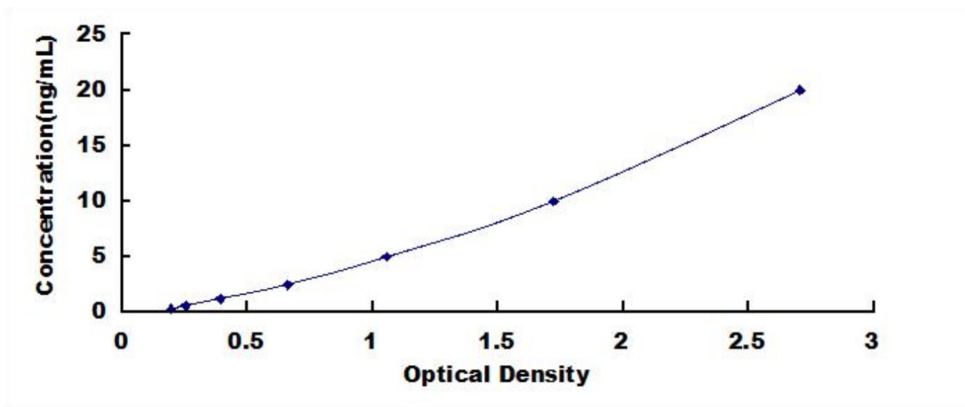
Typical Standard Curve for RUNX1, Rat ELISA.
