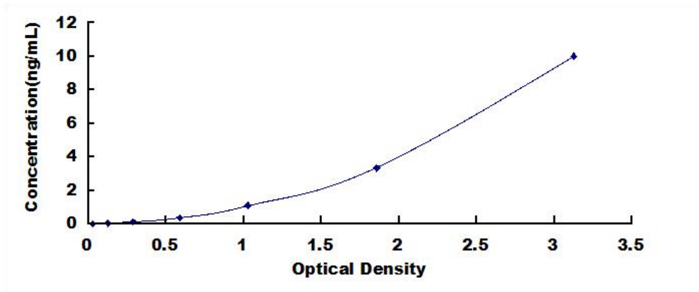
Typical Standard Curve for USP7, Human ELISA.
