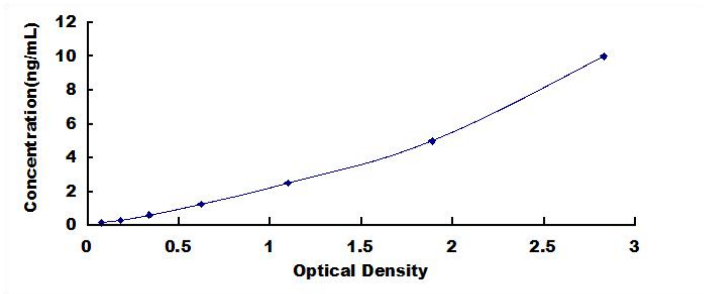
Typical Standard Curve for DOCK10, Human ELISA.
