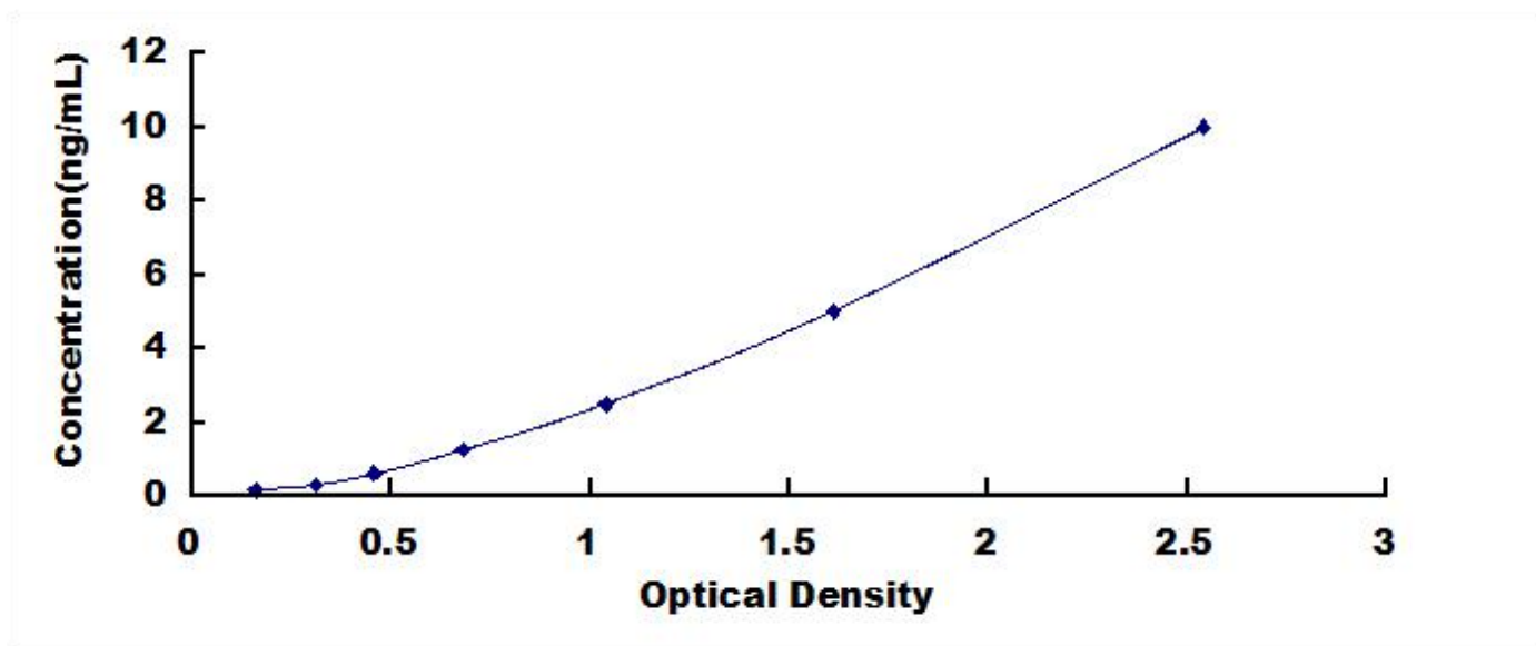
Typical Standard Curve for NOV, Rat ELISA.
