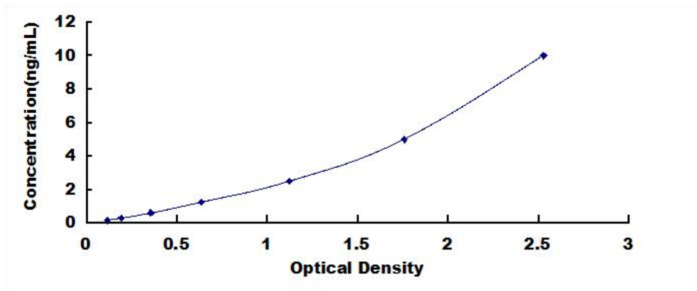
Typical Standard Curve for NRN1, Mouse ELISA.
