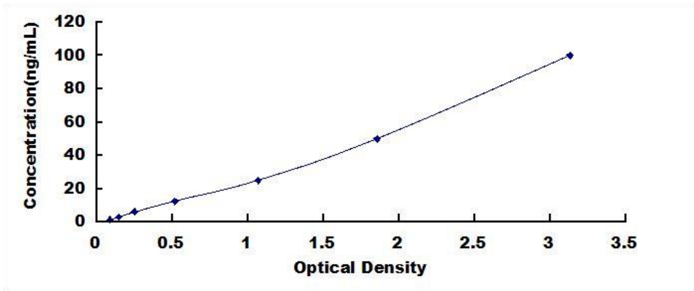
Typical Standard Curve for CA6, Mouse ELISA.
