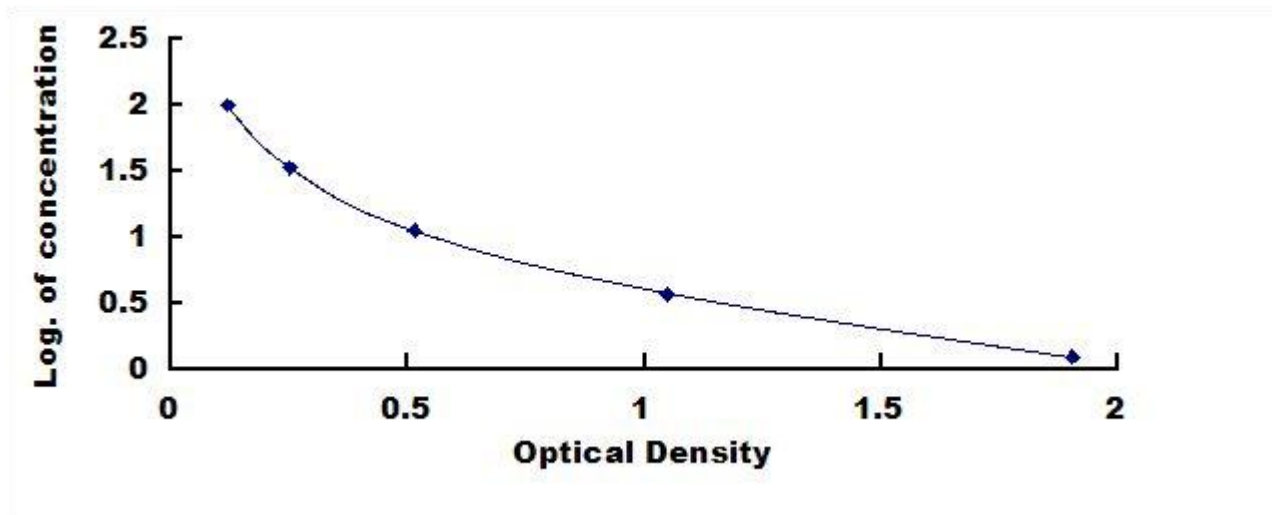
Typical Standard Curve for NT ELISA.
