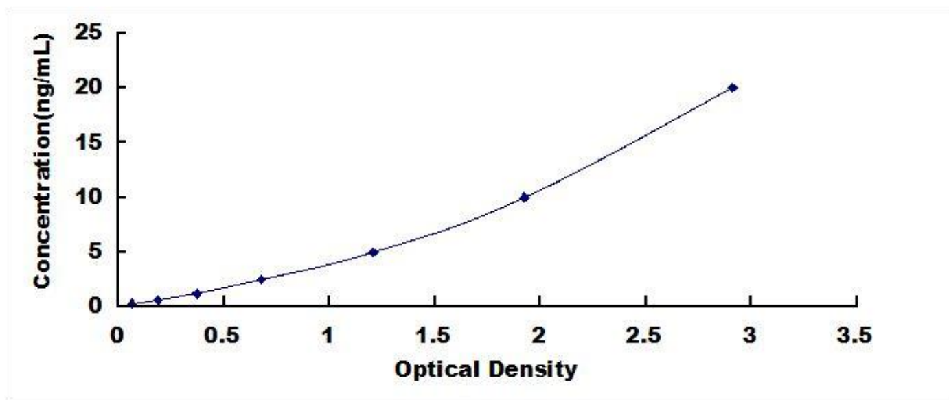
Typical Standard Curve for FNBP1, Mouse ELISA.
