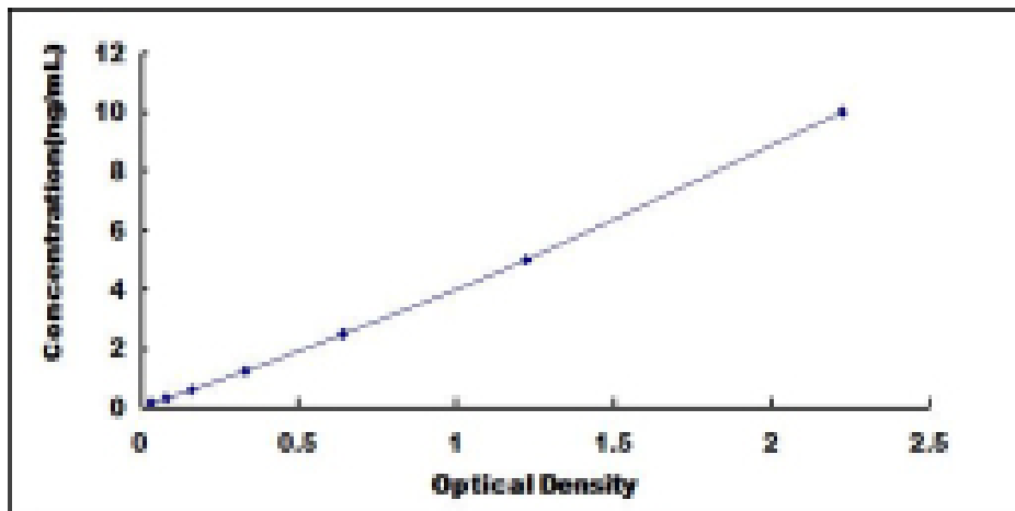
Typical Standard Curve for ACHAP ELISA.
