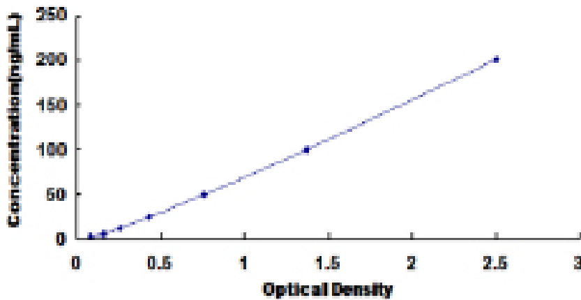
Typical Standard Curve for ADIPOR1 ELISA.
