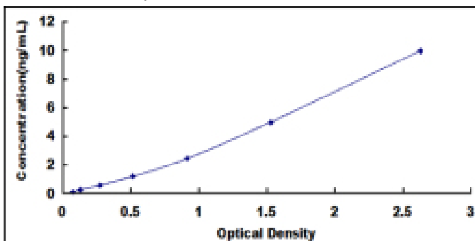
Typical Standard Curve for AADAT ELISA.
