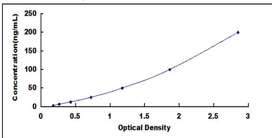
Typical Standard Curve for AT ELISA.
