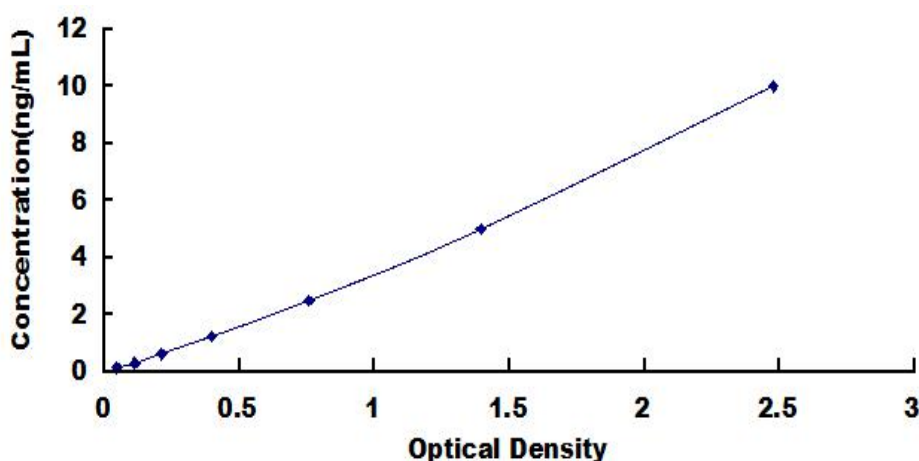
Typical Standard Curve for Bid ELISA.
